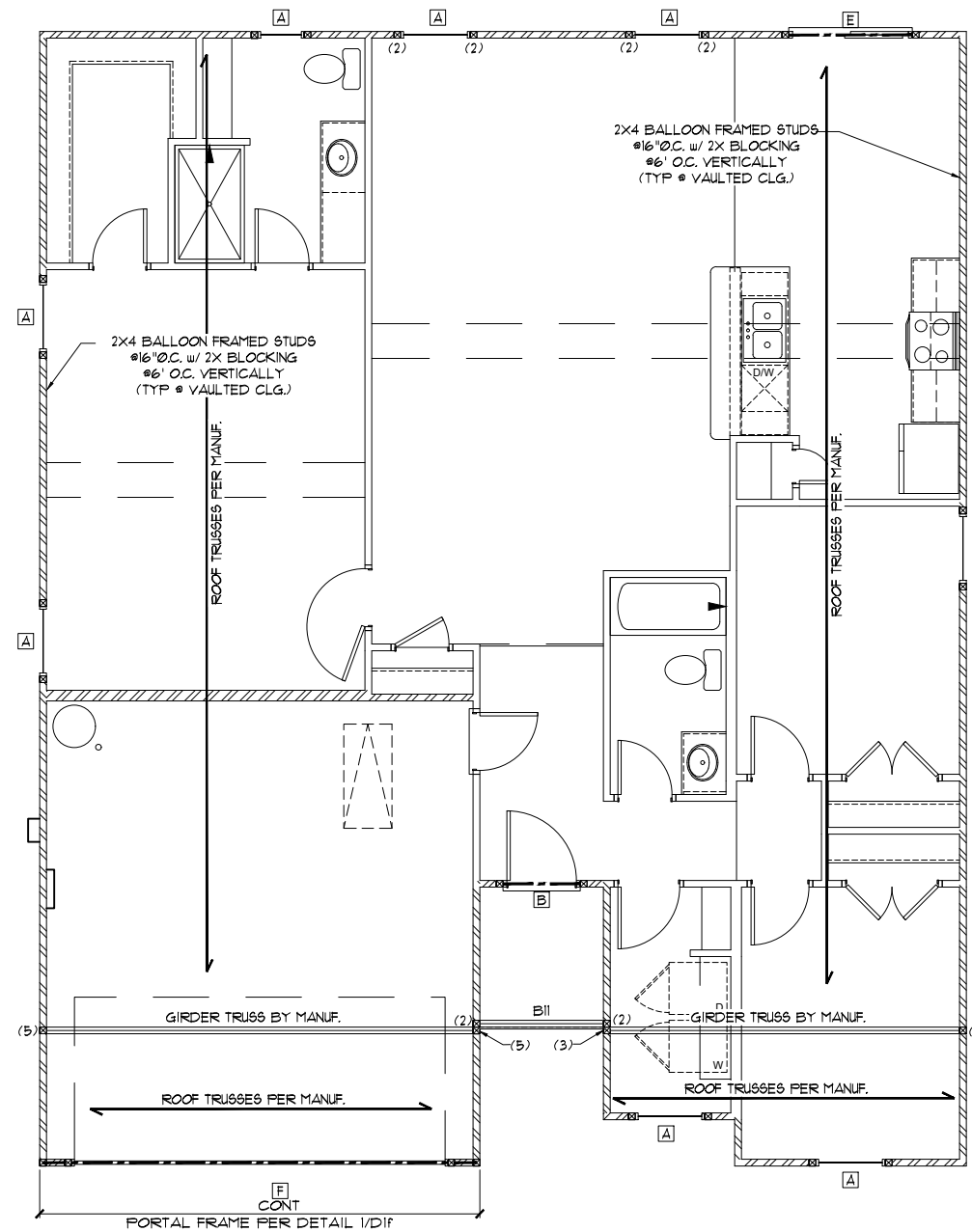
ALL ELEVATIONS - ROOF TRUSSES
