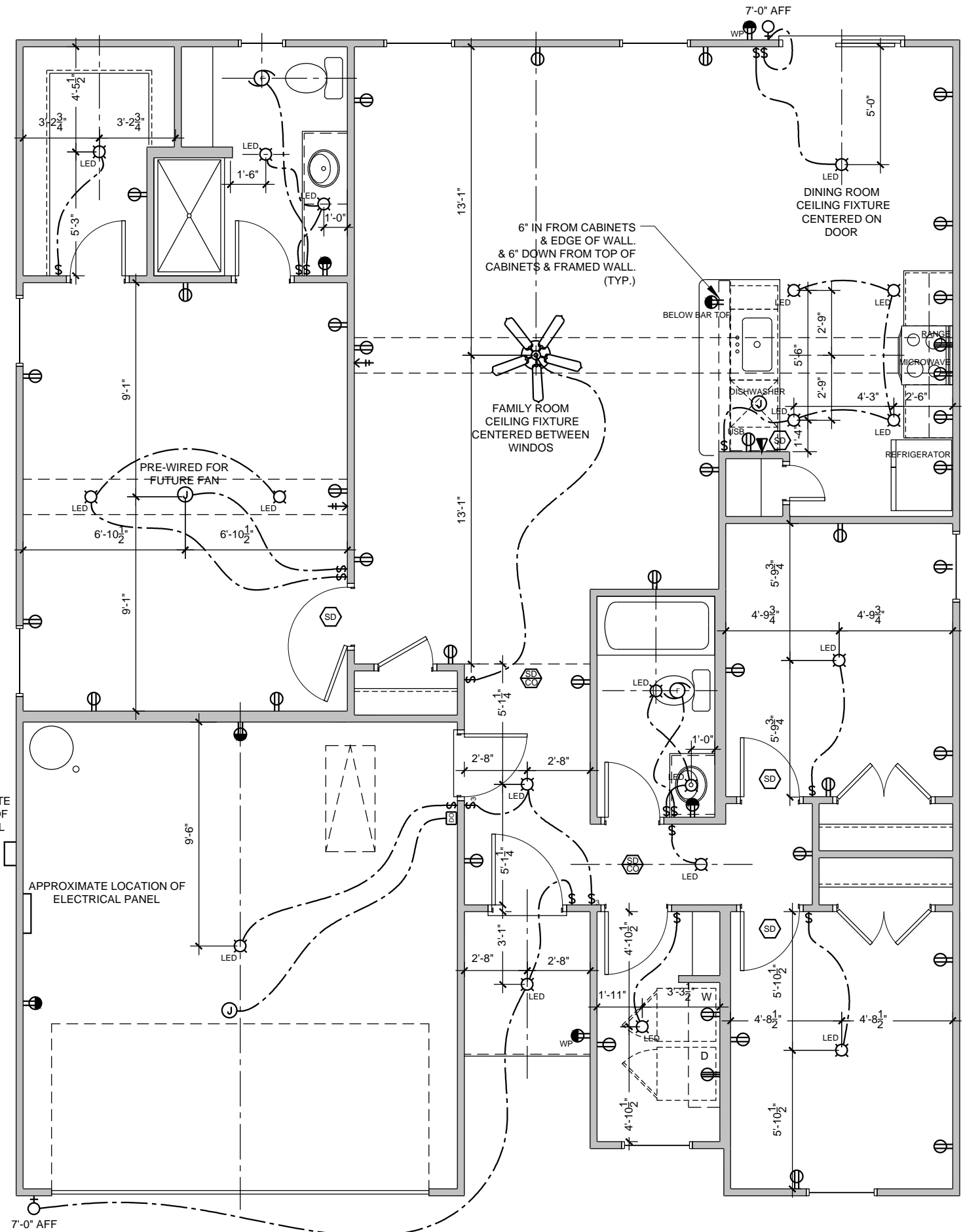
1 ELECTRICAL PLAN 3/16" = 1'-0"
