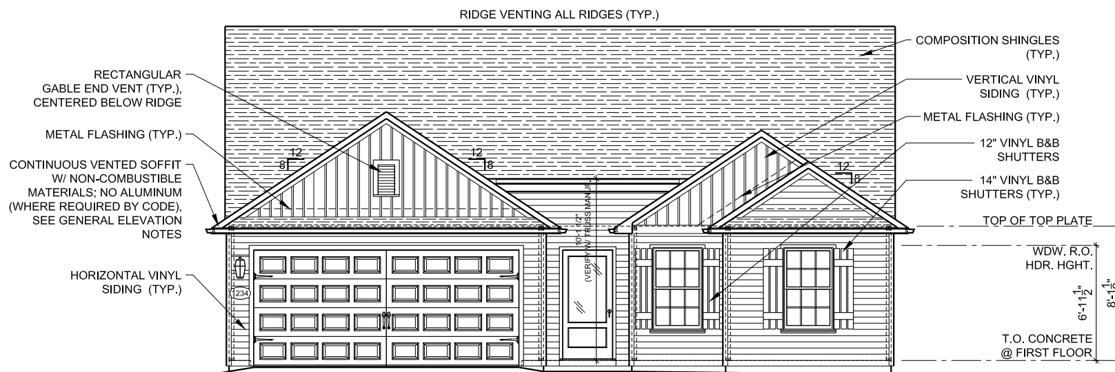
1 FRONT ELEVATION 1/8" = 1'-0"
